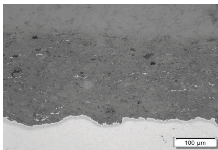
Typical microstructure of AZ Supra sprayed with our Master Jet® flame spray gun.
